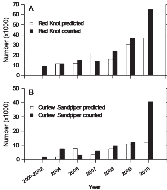
Figure 7. Predicted and counted peak numbers of Red Knot (A) and Curlew Sandpiper (B) in the core study area (Beipu, Nanpu and Zuidong) (including 67 km 2 of tidal flats) in Tangshan during northward migration from 2000 to 2010. The white and black bars give the predicted and counted peak numbers at the core study sites in 2000-2002, 2004 and 2006-2010 respectively.
